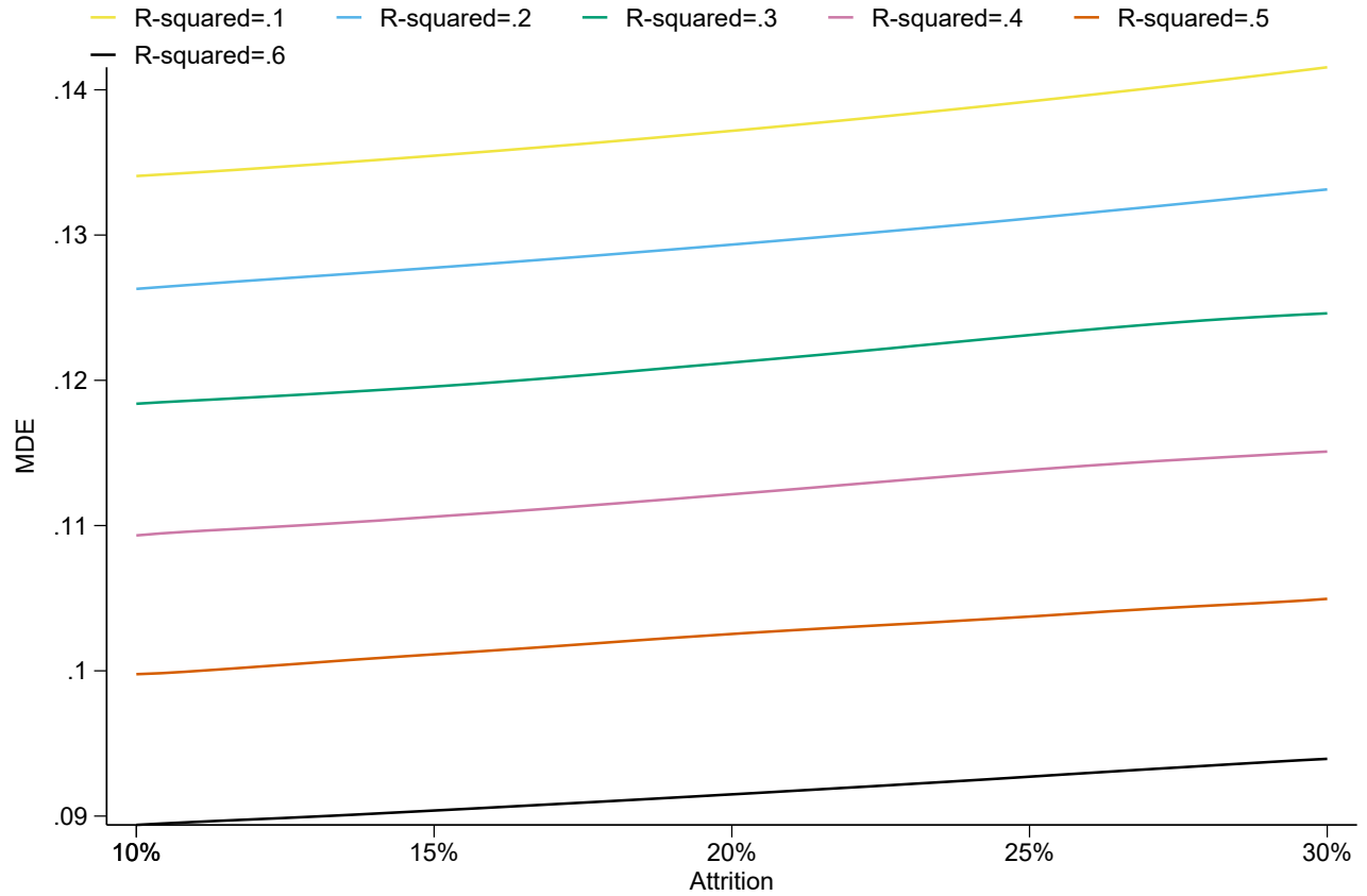
Figure 1: Power calculations
